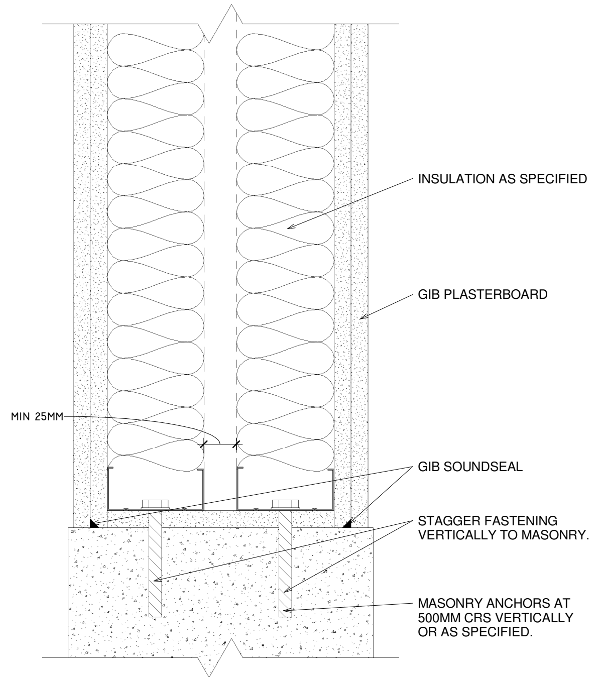
DOUBLE SRP STEEL STUD TO MASONRY WALL CONNECTION
