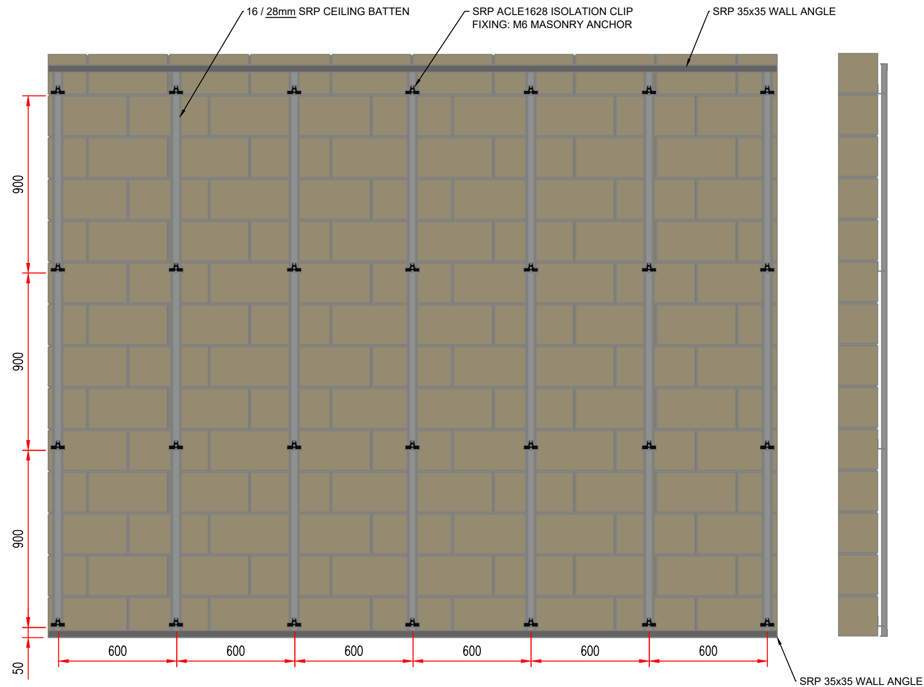
STANDARD SRP WALL STRAPPING SYSTEM 16/28 BATTEN WITH ADJUSTABLE WALL FIX CLIP + WALL ANGLE
