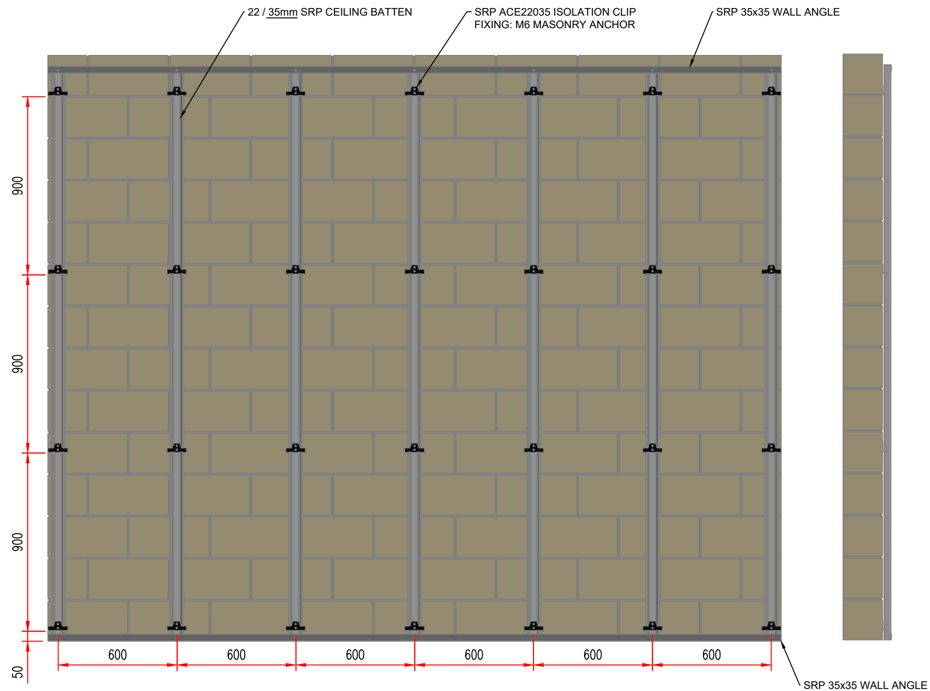
STANDARD SRP WALL STRAPPING SYSTEM 22/35 BATTEN WITH ADJUSTABLE WALL FIX CLIP + WALL ANGLE
