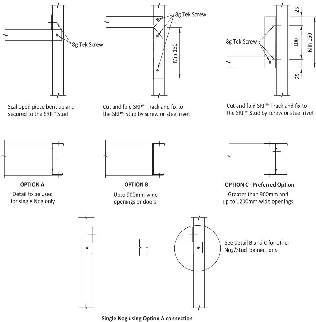
FIGURE 14 SRP™ Single Steel Nog Track Details
