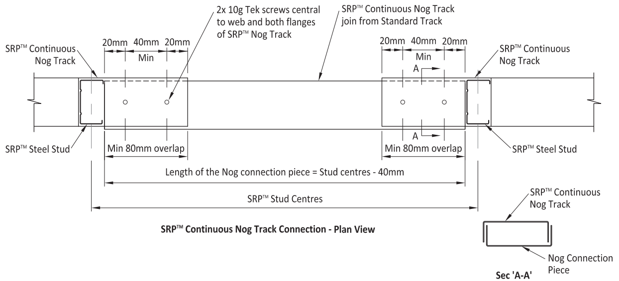
FIGURE 17 SRP™ Continuous Nog Track
